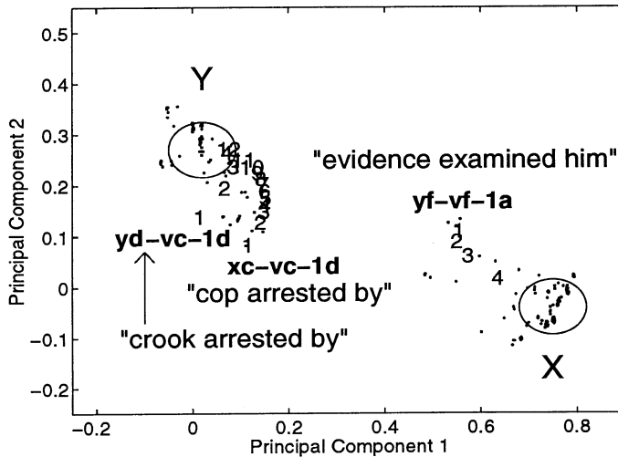
Figure 6. Three trajectories in the “1” region. (See previous figure for explanation of labels.)
