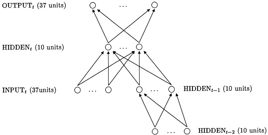
Figure 1. Three layer network with recurrent connections in the hidden layer (implemented as partial unfolding across time).
