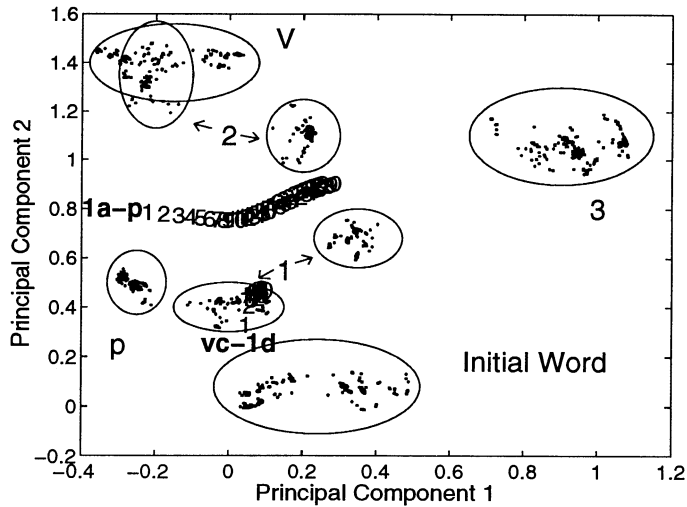
Figure 7. Trajectories for a semantic anomaly (labeled 'vc-1d' and a syntactic anomaly (labeled '1a-p'). The semantic anomaly occurs at the word '1d' in the sentence 'xc-vc-1d-2d-3d-p'. The syntactic anomaly occurs at the word 'p' in the string 'xb-va-1a-p'.
