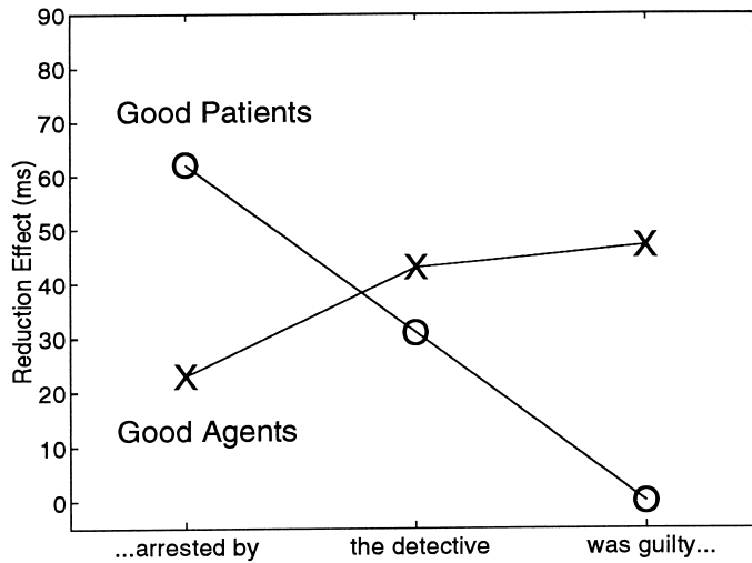
Figure 2. Crossed and smoothed latencies in the main clause/reduced relative ambiguity (after McRae et al. (in press)). The "X" sentences began with "Good Agents"; the "O" sentences began with "Good Patients".
