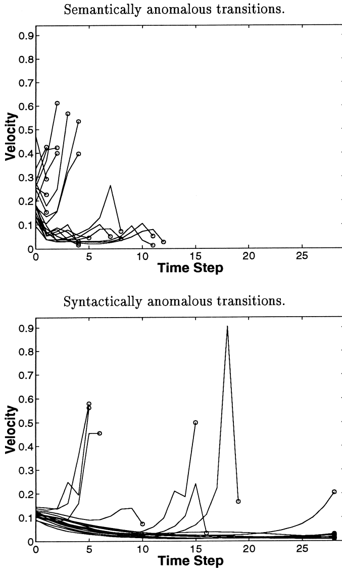
Figure 8. Velocity profiles for 20 semantically and 20 syntactically anomalous transitions. The profile is pictured for either the word at which the anomaly occurred or the word following this word, whichever had a longer gravitation time.
